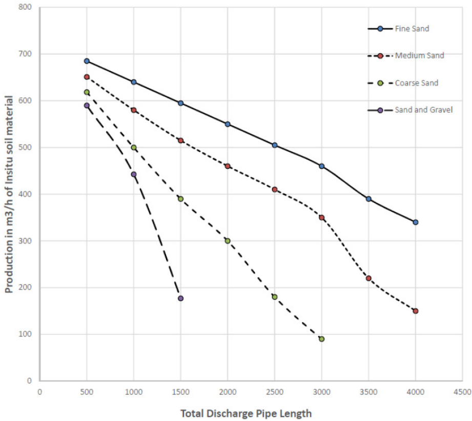
CSD450 Production Curve
