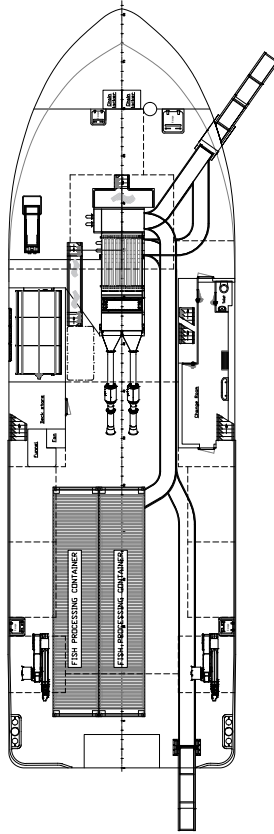
Main Deck
